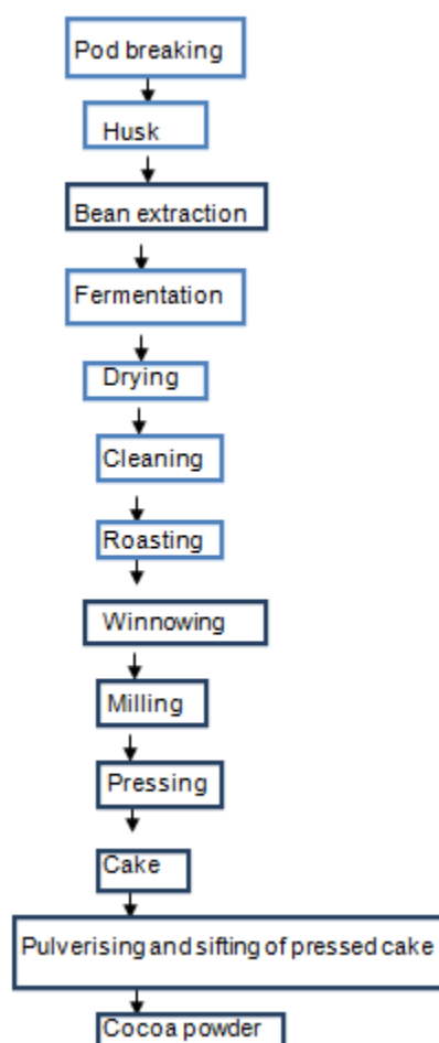
Fig. 1. Flow chart for cocoa powder
