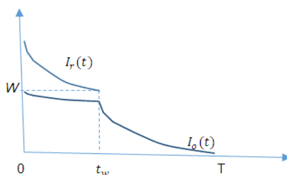
Fig. 1. Graphical representation of the model
