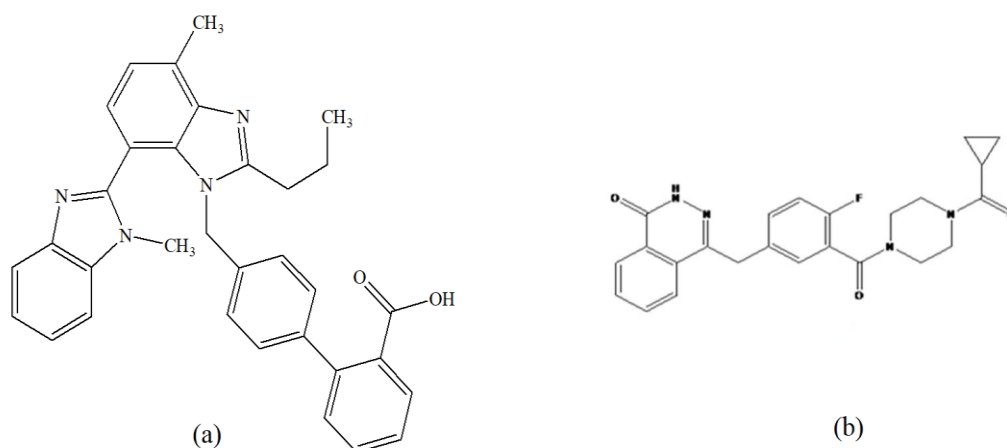
Fig. 1. Chemical structure of telmisartan (IS, a) and olaparib (b).
