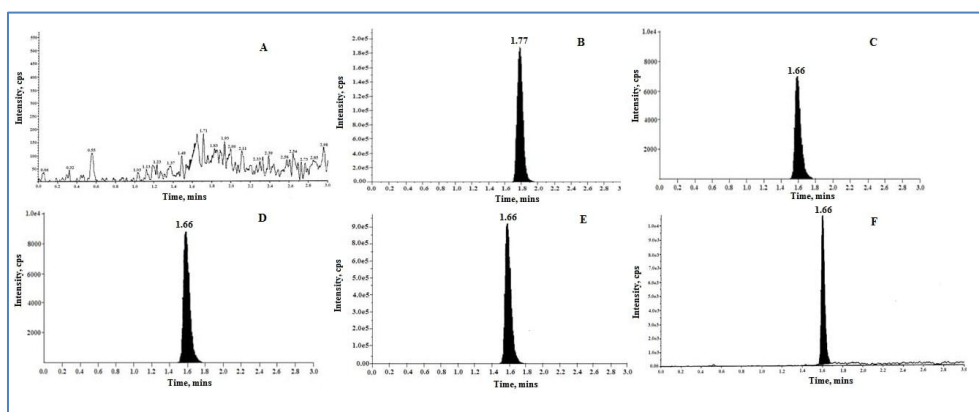
Fig. 3. Representative MRM chromatograms of olaparib and IS in rat plasma. A) Blank plasma; B) Blank plasma spiked with an internal standard, 200 ng/mL; C) Plasma spiked with olaparib at 1.00 ng/mL (LLOQ); D) Low quality control sample E) Upper limit of quantitation F) A rat plasma obtained at 25 mins after IV administration, 1 mg/kg
