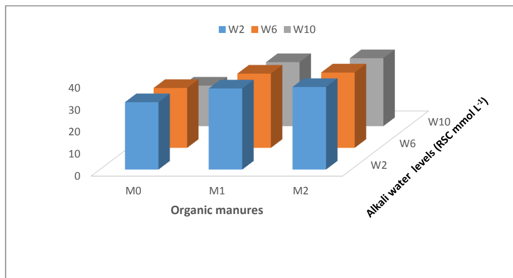
Fig. 2. Interactive effect of application of alkali water and organic manures on grain yield of wheat (Pooled)
