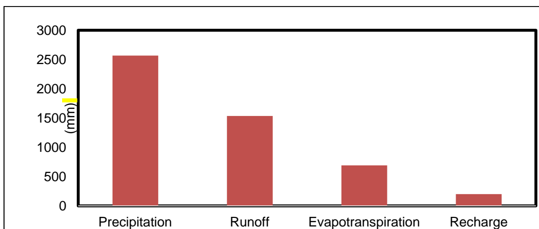
Fig. 4. Average annual water balance components in mm (1992-2019)
