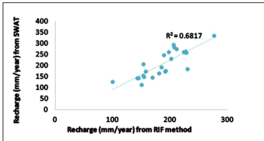
Fig. 6. Recharge obtained from SWAT model versus RIF method
