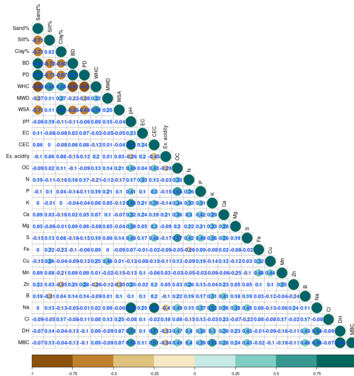
Fig. 5. Correlogram showing Pearson's correlations between the various properties of coastal sandy soils of AEU 1, Thiruvananthapuram district
