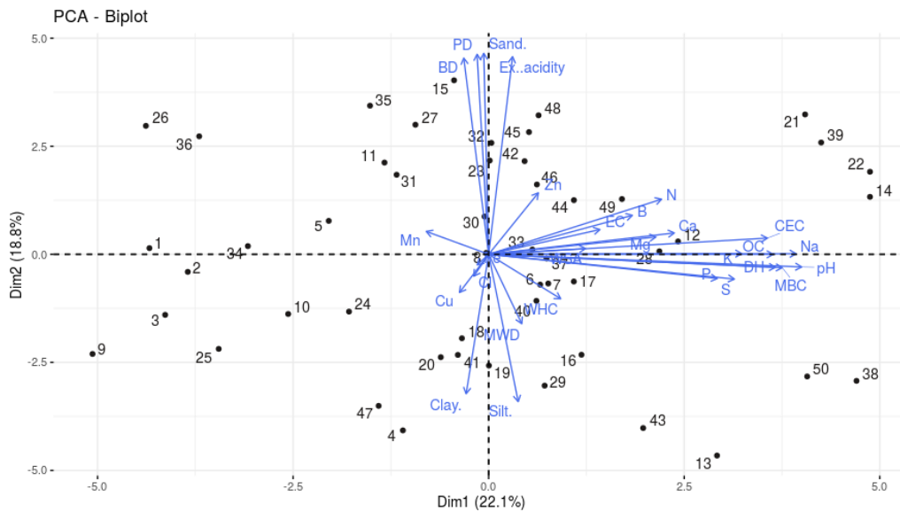
Fig. 2. Principal component analysis biplot with properties of coastal sandy soils of AEU 1, Thiruvananthapuram district
