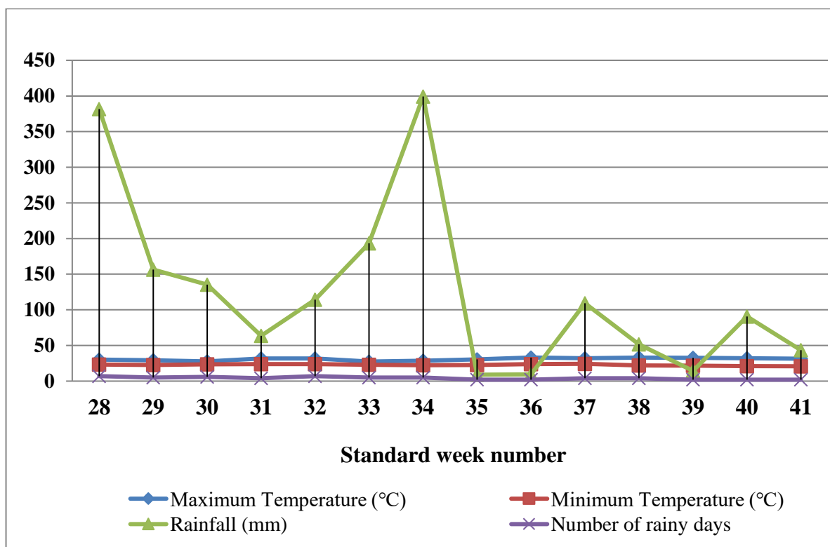
Fig. 1. Weekly meteorological data recorded at Sehore (M.P.) during crop season (From 9th July to 14 October 2022)
