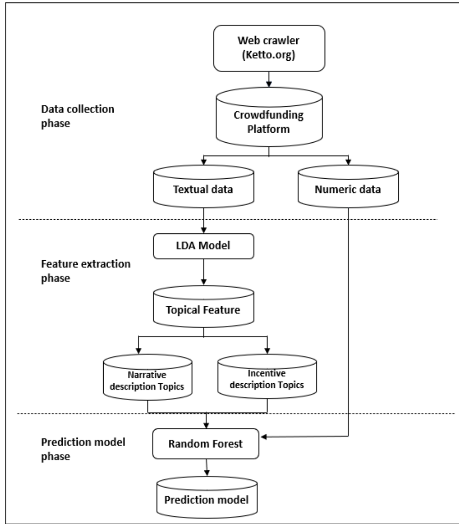
Fig. 1. LDA Semantic text analytics artifact
