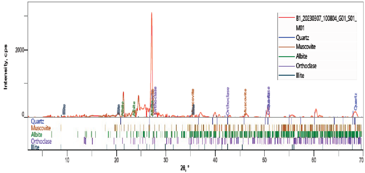
Fig. 7. XRD Pattern of Ekim Itam Calcined Kaolin
