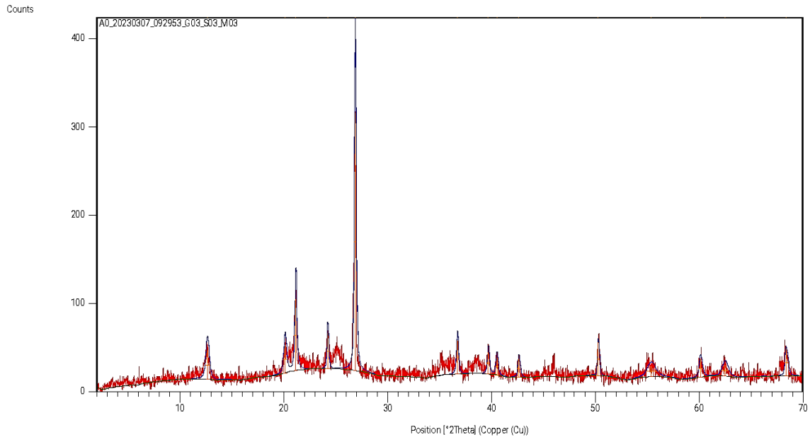
Fig. 1. XRD Pattern of Ikot Uso Akpan Itam Untreated Kaolin
