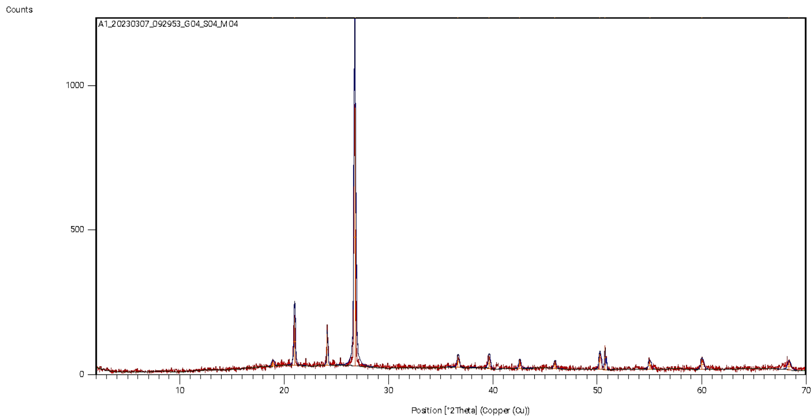
Fig. 3. XRD Pattern of Ikot Uso Akpan Itam Calcined Kaolin
