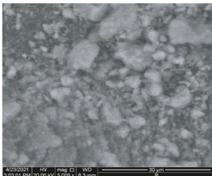
Fig. 9. SEM Micrograph of Raw (Untreated) Ikot Uso Akpan Itam kaolin at 500x magnification
