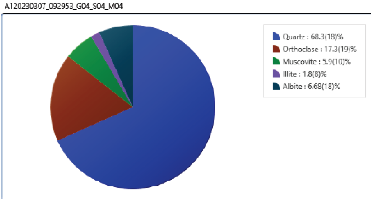
Fig. 4. Percentage quartz, Orthoclase, Muscovite, illite and Albite in calcined kaolin from Ikot Uso Akpan Itam Calcined Kaolin
