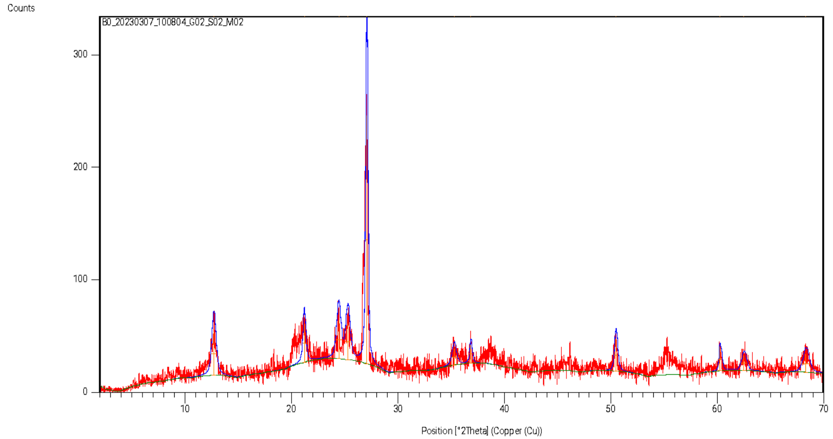
Fig. 5. XRD Pattern of Ekim Itam Untreated Kaolin
