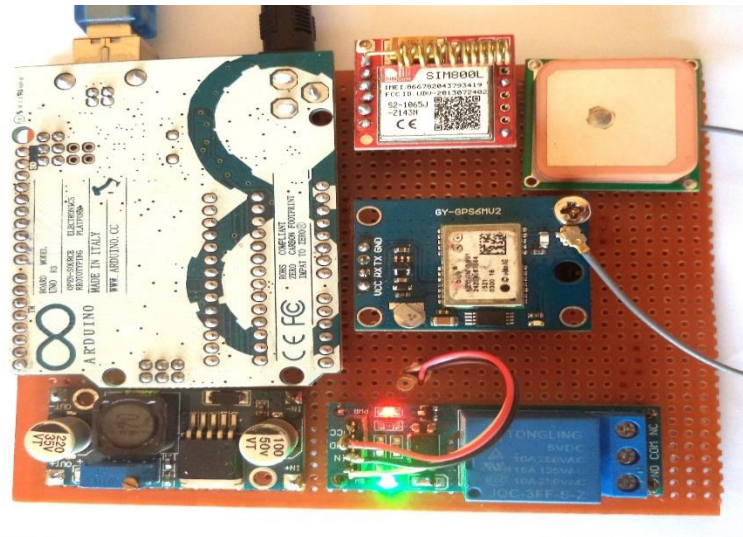
Fig. 9. A pictorial representation of the assembled components
