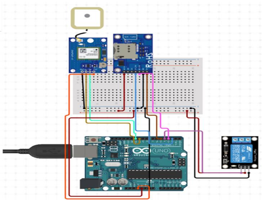
Fig. 8. A complete circuit diagram of the GPS-GSM motorcycle security system
