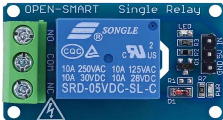
Fig. 6. A Relay board 5v 1 – Channel single relay module
