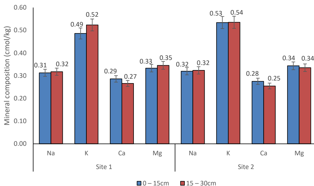
Fig. 1. Mineral composition of the two studied depths and sites
