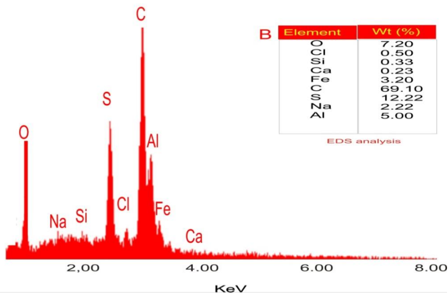
Fig. 1. EDX micrograph of carbon dot from coconut shaft
