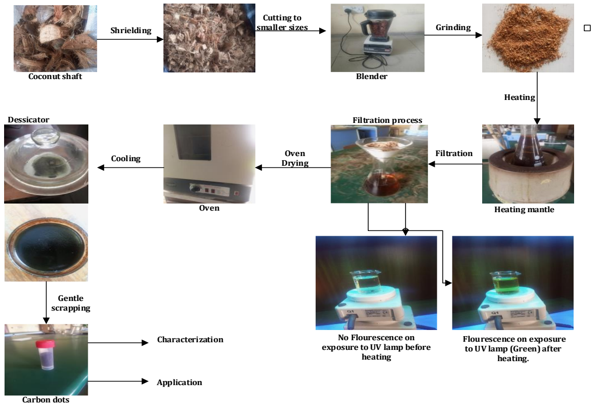
Plate 3. Synthesis of Carbon dots (C-dots) from coconut shaft using hydrothermal method
