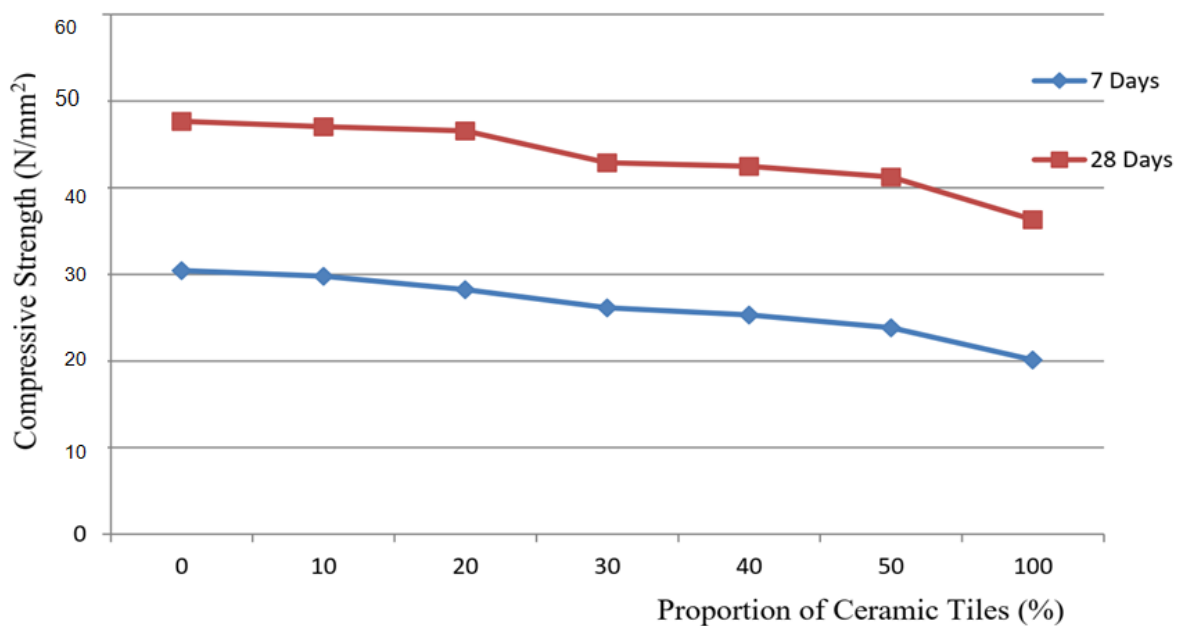
Fig. 15. Compressive strength of concrete for varying proportion of ceramic tiles
