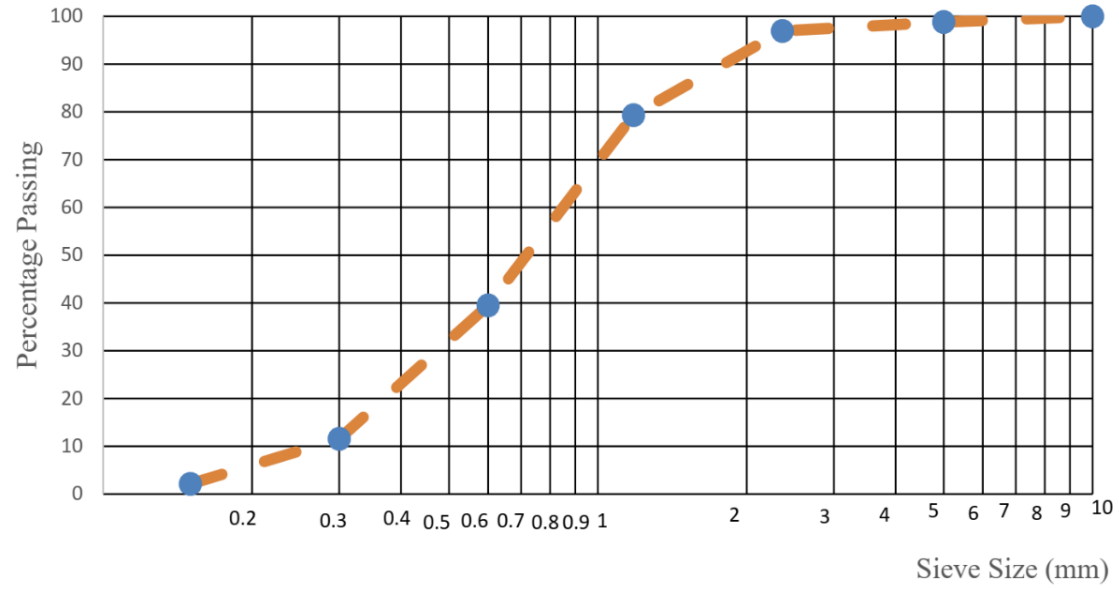
Fig. 11. Particle size distribution curve for sand
