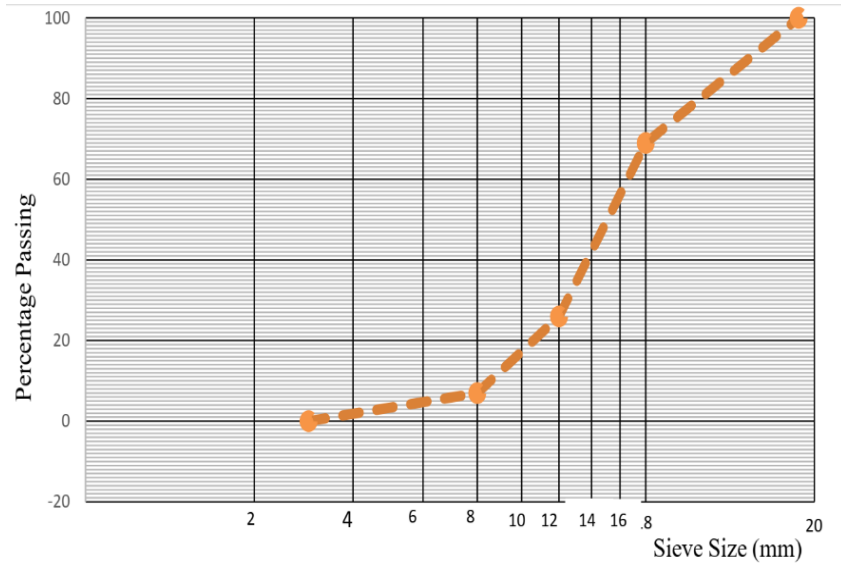
Fig. 9. Particle size distribution of crushed granite
