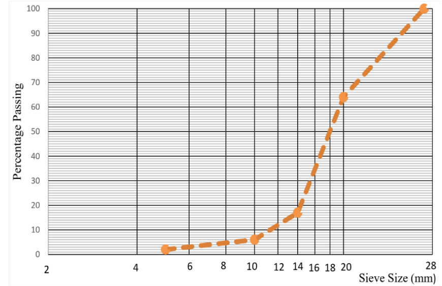
Fig. 10. Particle size distribution curve for waste ceramic tile
