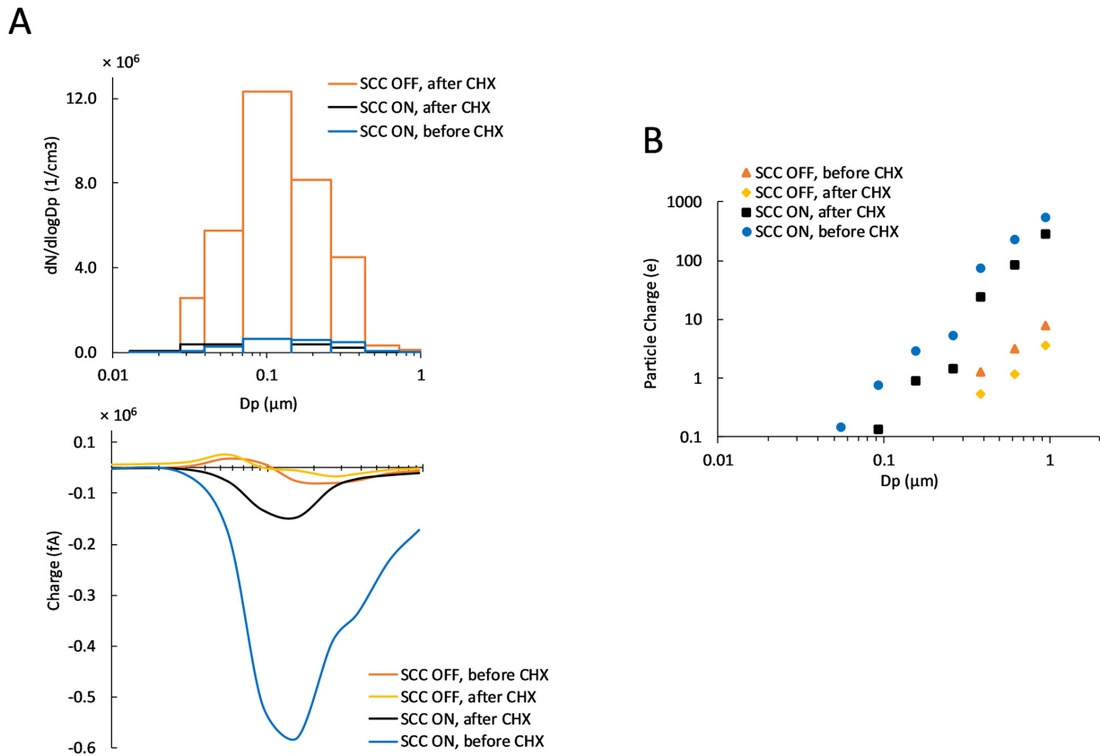
Figure 8. (A) Comparison of particle number and charge size distributions before and after the condensing heat exchanger (CHX) with particle charging on and off and (B) single particle charge distribution.
