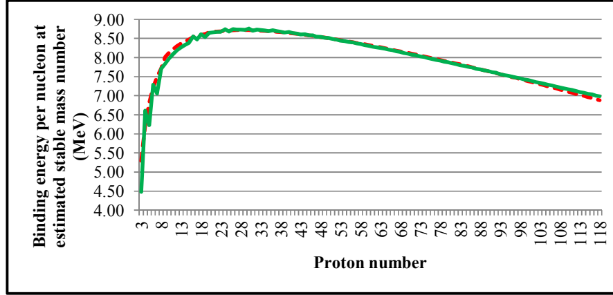
Fig. 1. Binding energy per nucleon close to stable mass numbers of Z = 3 to 118
