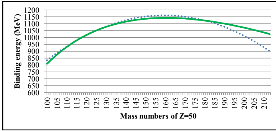
Fig. 2. Isotopic binding energy of Z=50
