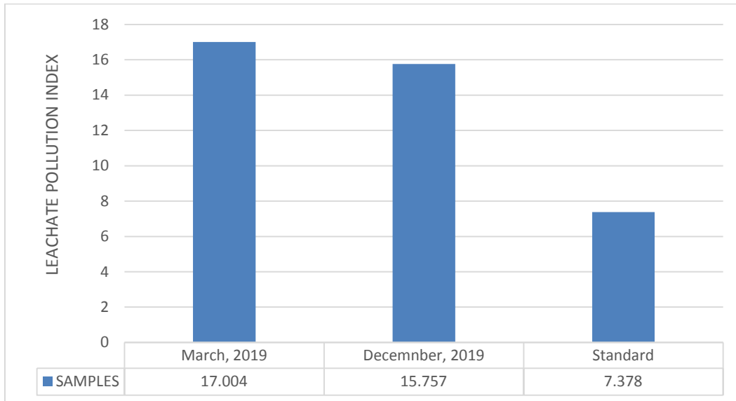
Fig. 1. Leachate Pollution Index at YCWD
