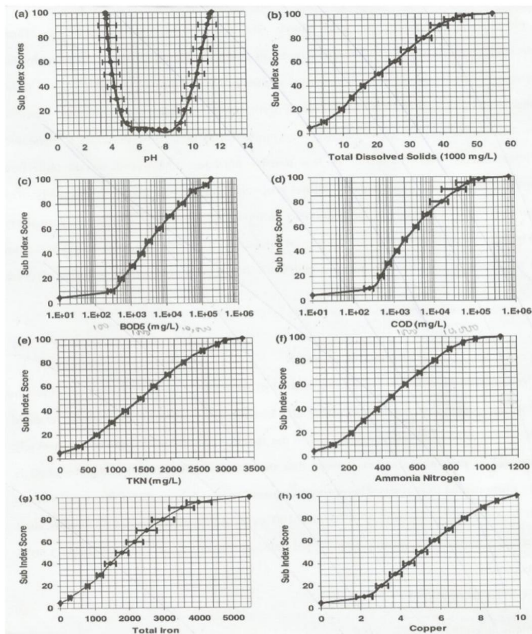
Fig. 2. The average sub-index curves of pollutants [13]
