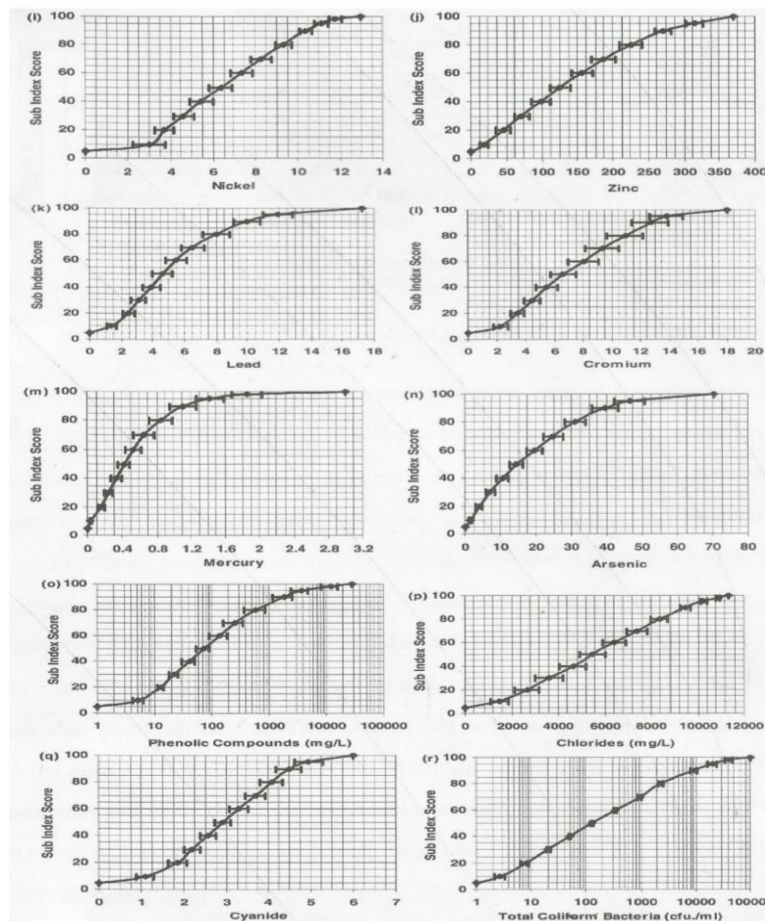
Fig. 3. The average sub-index curves of pollutants [13]
