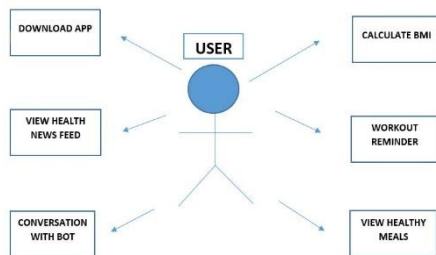
Fig.1. UML Diagram
