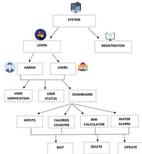
Fig.8. Block Diagram of MT (Muscle Town)
