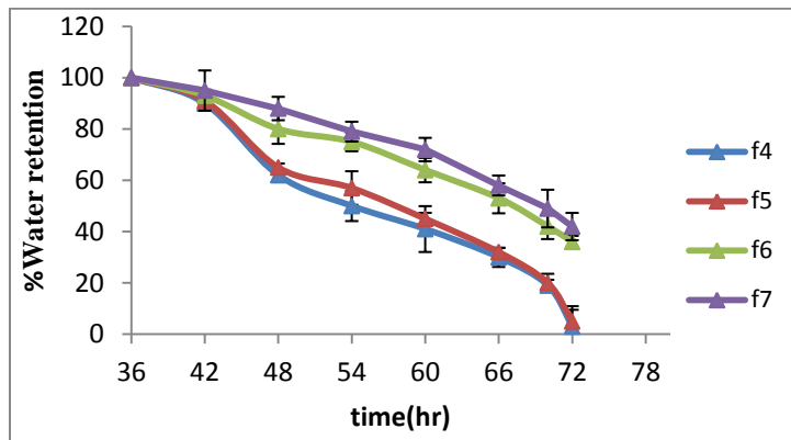
Fig. 4. Degradation of superporous hydrogel tablets. (n=3, mean±S.D)
