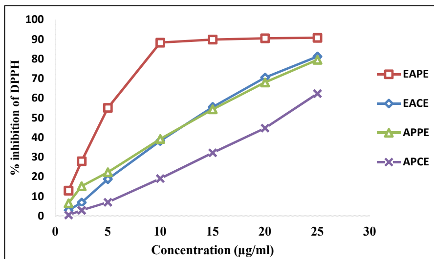
Fig. 1. Graph showing % inhibition activity of tested extracts in DPPH assay EAPE; E. angustifolia leaves processed extract, EACE; E. angustifolia leaves crude extract, APPE; A. pseudalhagi herb processed extract, and APCE; A. pseudalhagi herb crude extract
