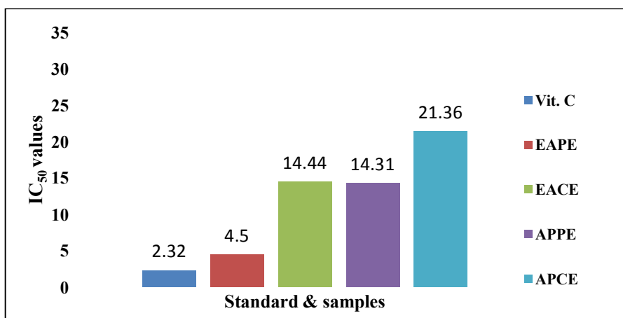
Fig. 2. Graph showing the IC 50 values for the standard and tested extracts Vit. C; vitamin C, EAPE; E. angustifolia leaves processed extract, EACE; E. angustifolia leaves crude extract, APPE; A. pseudalhagi herb processed extract, and APCE; A. pseudalhagi herb crude extract
