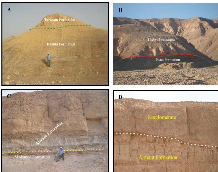
Figure (4): Field Photograph showing Tarawan Formation conformably underlaid by Dakhla Formation (A), Esna–Thebes boundary (B), Madamud–Armant Formation boundary (C) and Armant Formation–Fanglomerate disconformities boundary (D) at the study area.
