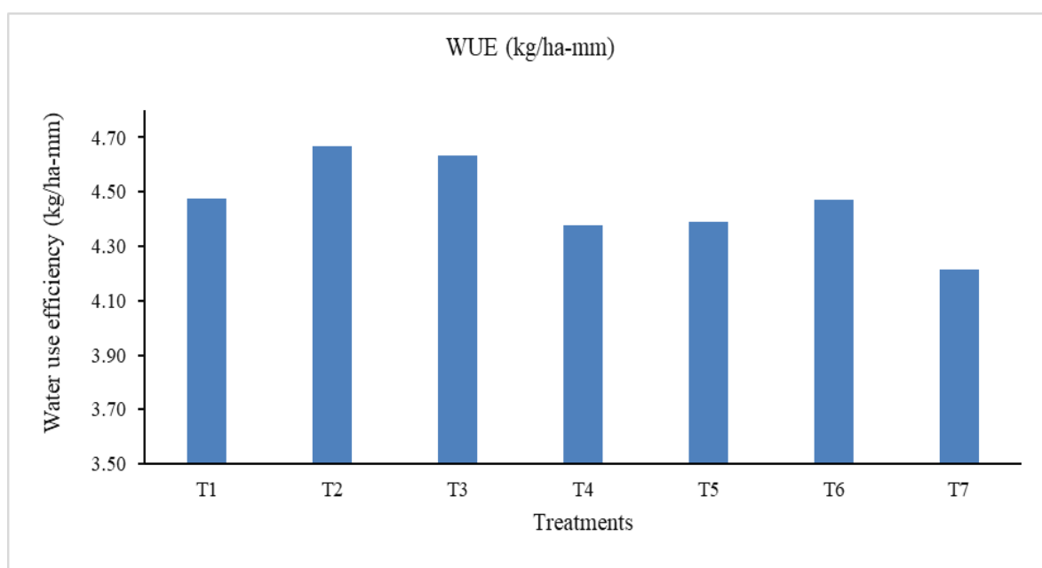
Fig. 6 Effect of silicon (Si) and different levels of surface irrigation water on Water use efficiency
