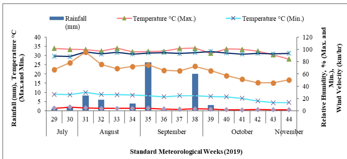
Fig. 2 Weekly meteorological data during crop season
