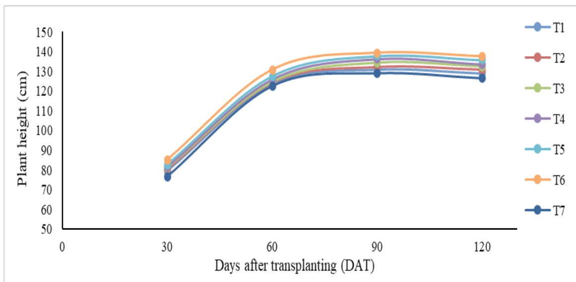
Fig. 3 Effect of silicon (Si) and different levels of surface irrigation water on plant height of rice crop under surface irrigation
