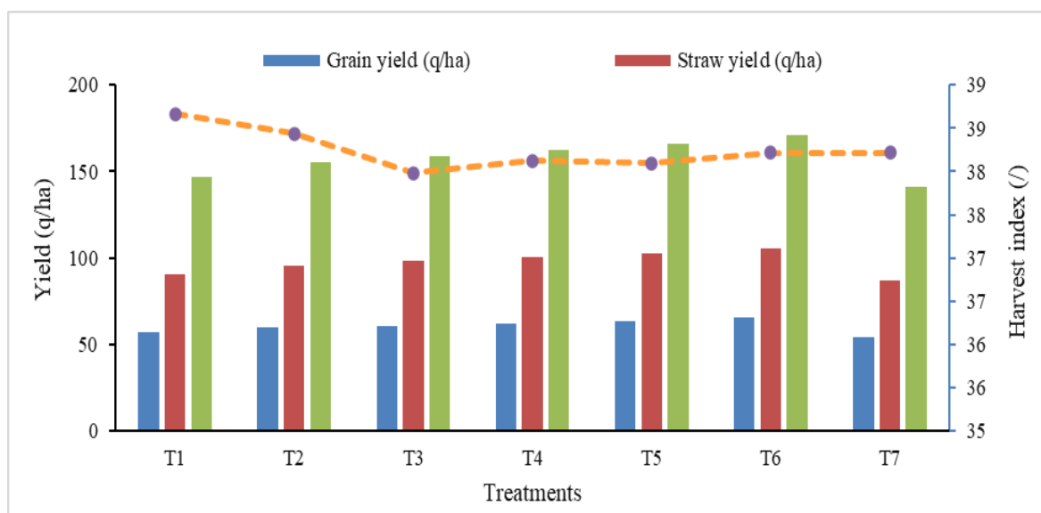
Fig. 5 Effect of silicon (Si) and different levels of surface irrigation water on grain, straw, biological yield and harvest index
