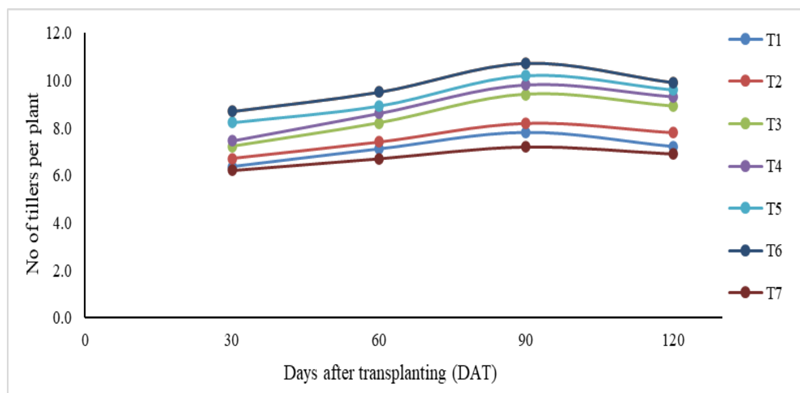
Fig. 4 Effect of silicon (Si) and different levels of surface irrigation water on number of tillers per plant on rice crop under surface irrigation
