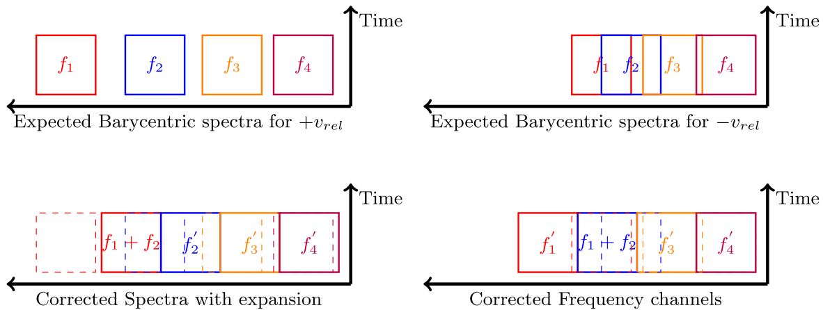
Figure A3. These plots depict the expected spectra at their respective barycentric frequencies and the spectra after the correction for barycentric relative velocity. Each plot represents a single spectrum, where the frequency increases from right to left. (a) In the case of +v_{rel} , the first channel of the topocentric spectra is shifted to a higher barycentric frequency compared to the last topocentric spectra channel, which causes an expansion of the spectra. If two consecutive channels move farther away from each other (shown as f_1 and f_2 ) by more than half the channel width, an additional channel is added in between, which is the summation of these two channels. Extra channels at the edge of the spectra are dropped. (b) In the case of -v_{rel} , the first channel of the topocentric frequency is shifted to a lower barycentric frequency relative to the last topocentric spectra channel, which causes a squeeze in the spectra. If two consecutive frequency channels shift closer to each other by more than half a channel width, these channels are added together and an extra channel is added at the end containing zeros. The bottom spectra in each plot illustrate these expansion and squeeze effects after correction are applied from the code.
