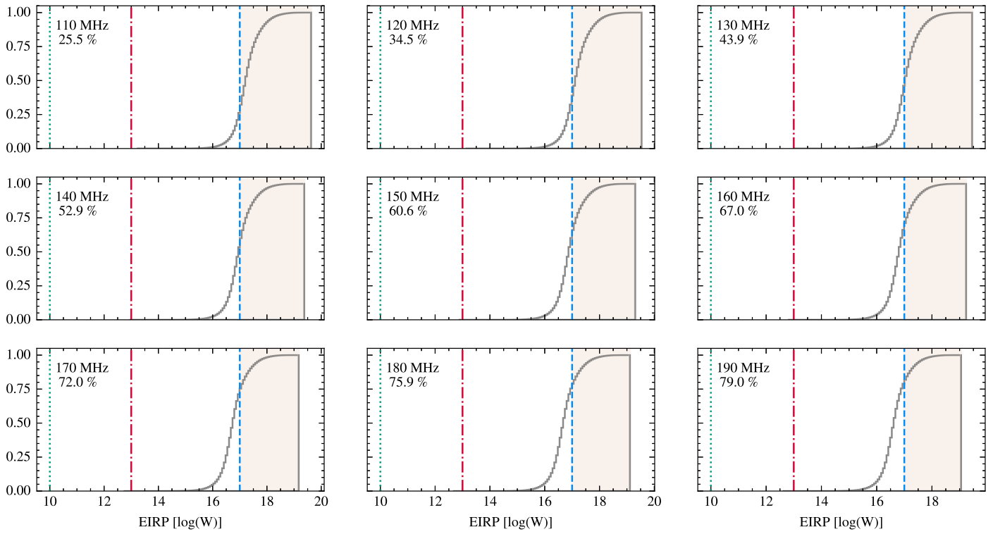
Figure 10. Cumulative histogram of EIRP limits of this survey across the HBA band. Reference luminosities for three civilization levels emitting 10^{17} , 10^{13} , or 10^{10} W are shown in blue, red, and green respectively. The percentage of targets where the station is sensitive to the transmission of 10^{17} W is shown, as a function of frequency across the band. At lower frequencies, sensitivity to 10^{17} emitters drops off as the T_{\text{sys}} rises. The T_{\text{sys}} varies from 1260 K down to 322 K as frequency is increased across the band. Detailed calculations are presented in Appendix B and Table B1.
