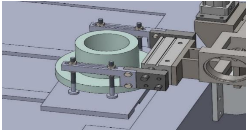
Fig. 4. Schematic diagram of gripping blank
