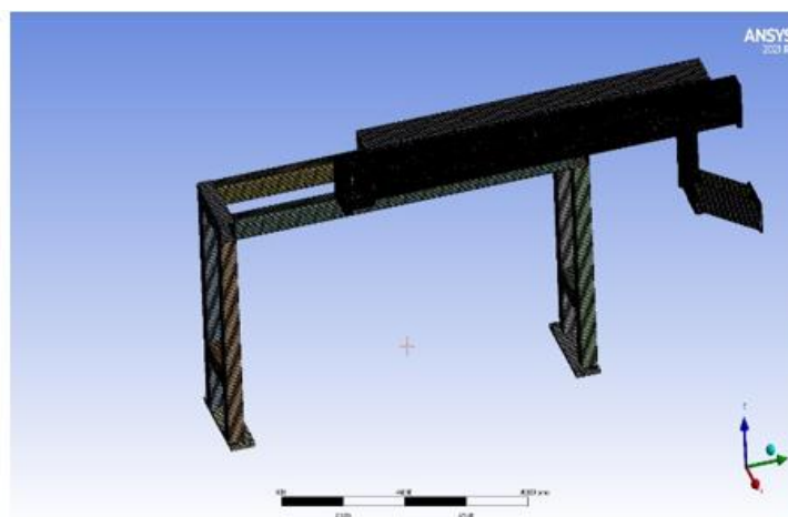
Fig. 6. Meshing of the model
