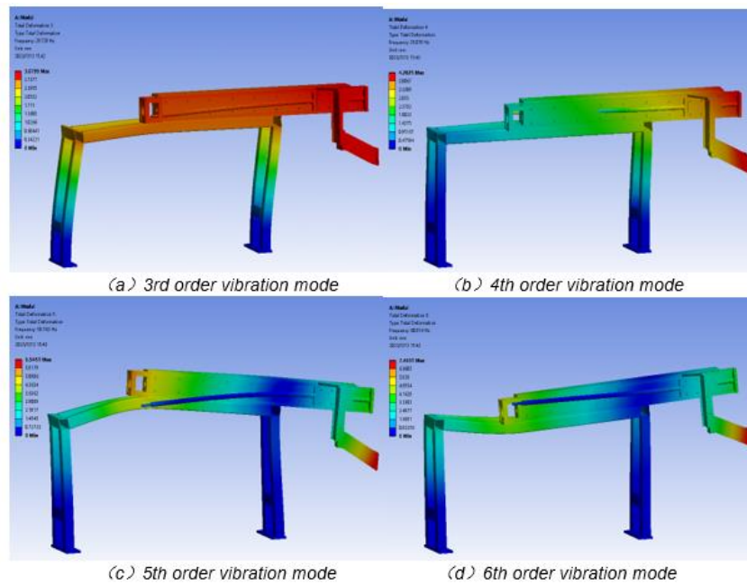
Fig. 9. Modal vibration pattern cloud
