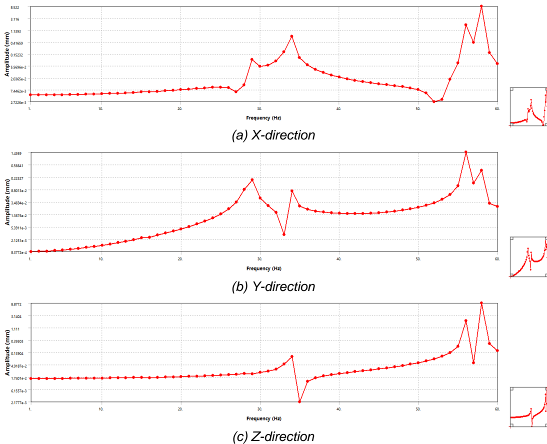
Fig. 11. Displacement response curve of the support frame in each direction
