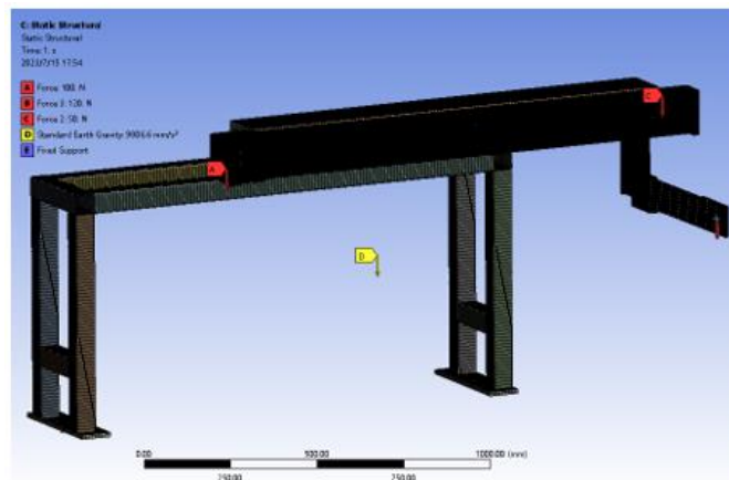
Fig. 7. Manipulator load force diagram
