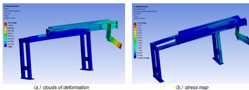
Fig. 8. Cloud diagram of deformation and stress distribution of the manipulator
