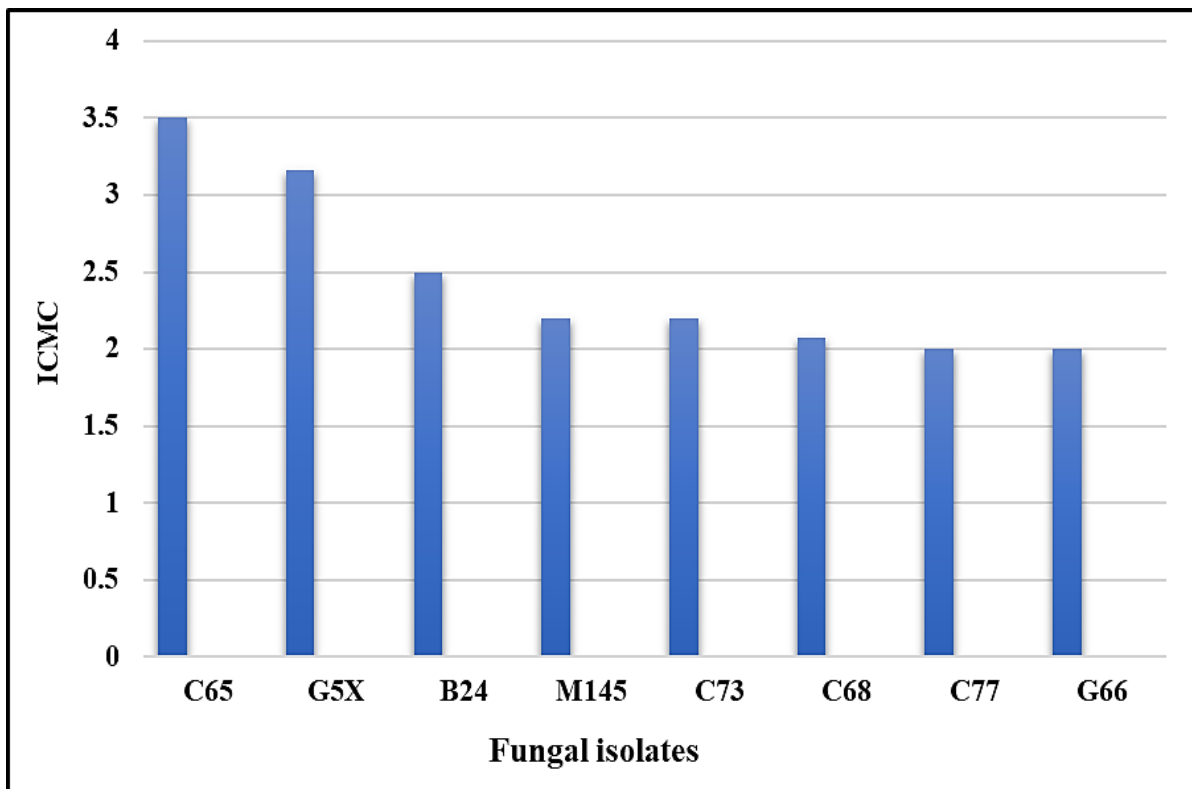
Fig. 2. Relative enzyme activity index (ICMC) of cellulose degrading fungal isolates isolated from forest soils of Maharashtra, India
