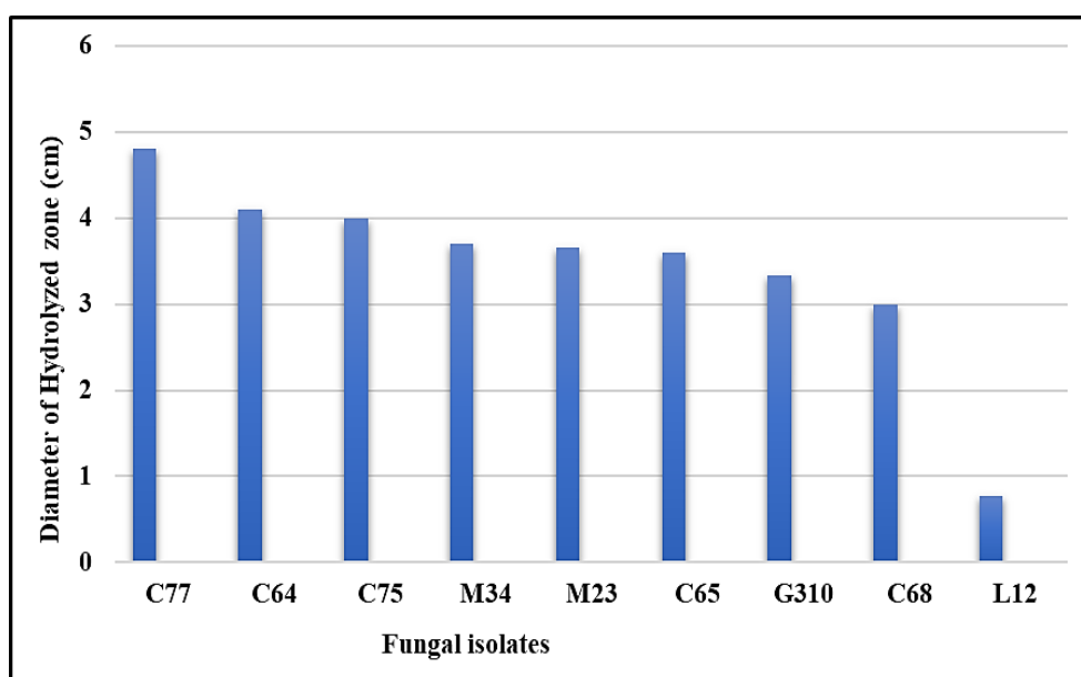
Fig. 1. Zone of hydrolysis by different fungal isolates
