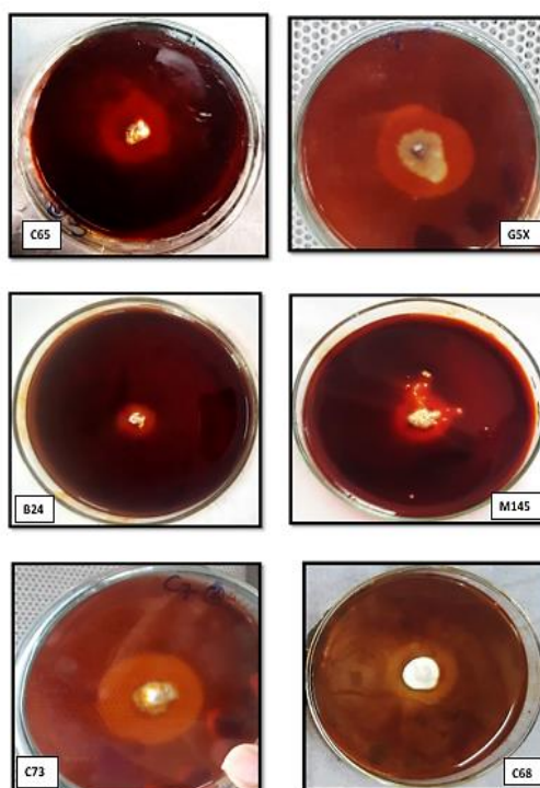
Plate 1. Screening of fungal isolates for cellulose degradation (Hydrolysis zone)
