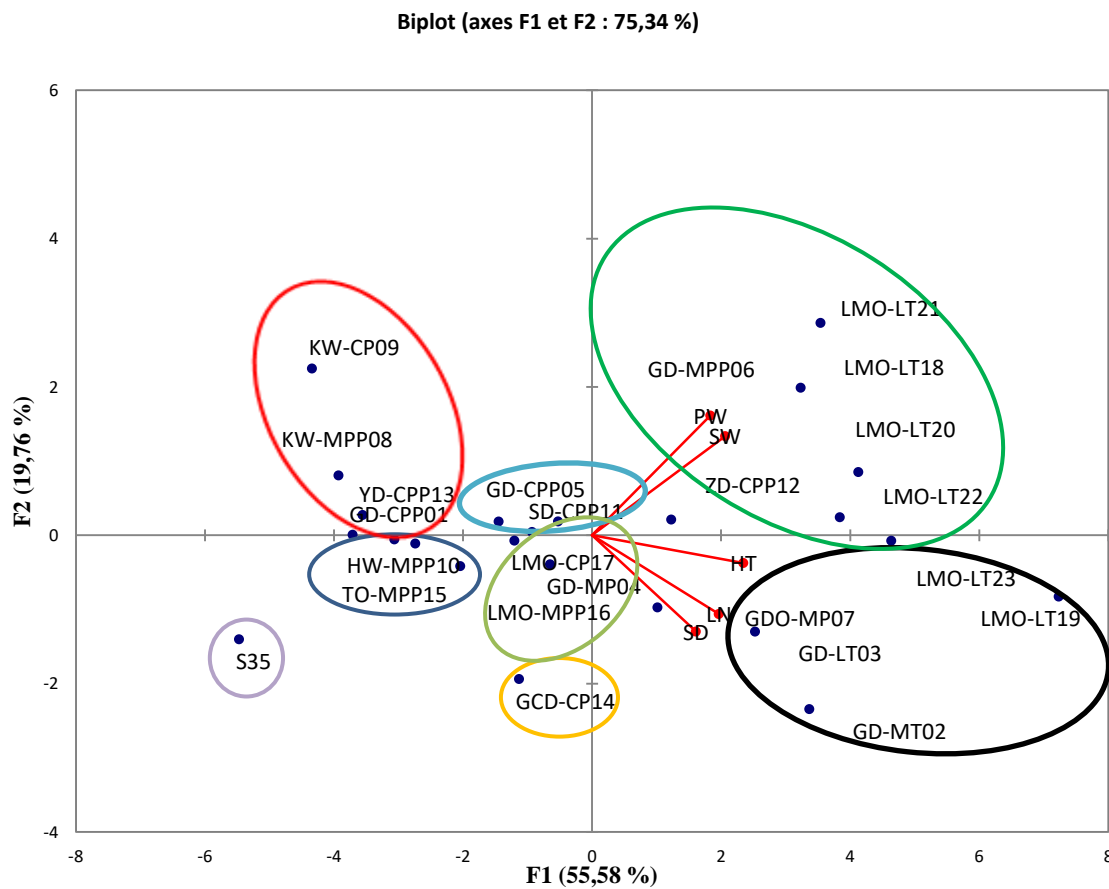
Fig. 2. Principal Component Analysis of affinity to quantitative parameters PW = Panicle weight; SW = Seed weight; HT = Height; LN = Leaves number; SD = Stem diameter
