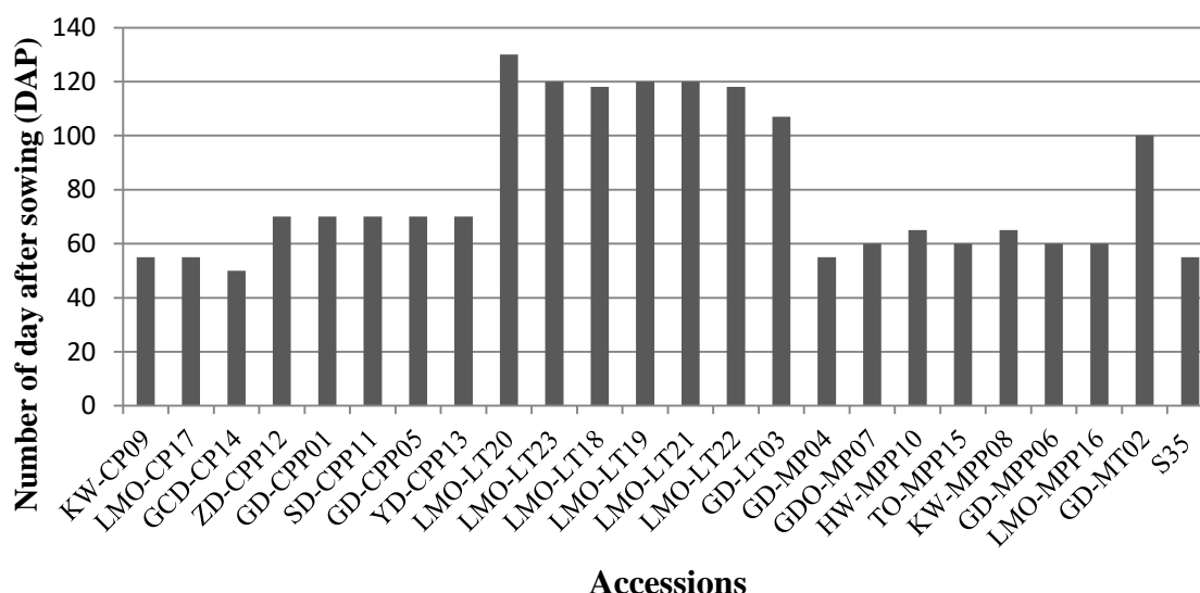
Fig. 3. Heading dates according to genotypes
