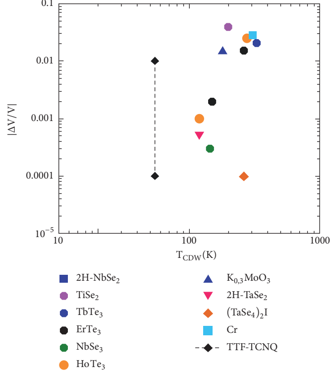
FIGURE 4: Color on line. Experimental discontinuities (absolute values) |\Delta V/V| of the velocity of the longitudinal C_{11} and C_{33} shown as a function of T_{CDW} (Tables 1 and 2). Results obtained with TbTe_3 (blue circle T_{CDW} = 330 K) [41], ErTe_3 (black circles T_{CDW1} = 260 K and T_{CDW2} = 155 K) [42], and HoTe_3 (brown circles T_{CDW1} = 280 K and T_{CDW2} = 120 K) [43]. Results obtained by Young and velocity measurements NbSe_3 (green circle) [27], 2H-NbSe_2 (blue squares) [16, 17], TiSe_2 (violet circle) [20], 2H-TaSe_2 (red down triangle) [16], K_{0.3}MoO_3 (blue up triangle [31]), (TaSe_4)_2I (brown diamond) [39], TTF-TCNQ (black diamonds) with a large discrepancy ( \sim 0.0001, 0.01 ) shown by the dotted black line [36, 37]), and Cr (light blue [54]).
