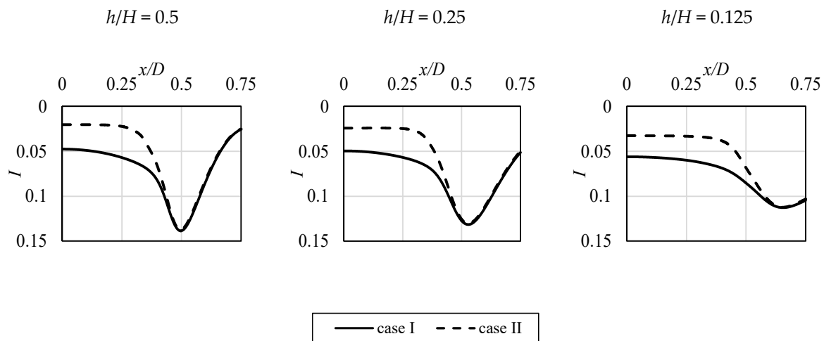
Figure 18. Impinging jet turbulence intensity profiles at various values of non-dimensional distance h/H above the impinging surface.
