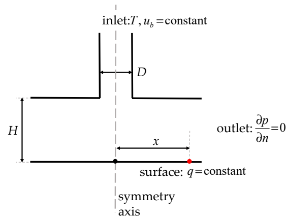
Figure 1. Boundary conditions placement. Indication of important geometrical variables. Further explanation is included in Table 2.
