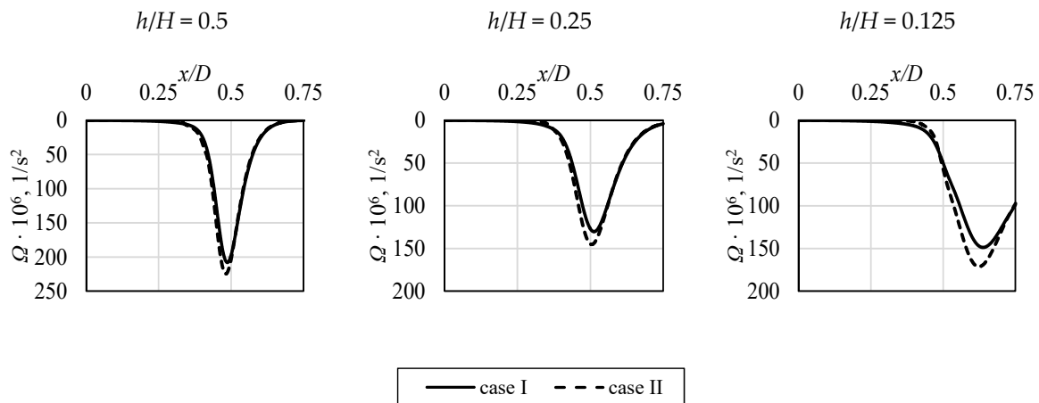
Figure 19. Impinging jet enstrophy profiles at various values of non-dimensional distance h/H above the impinging surface.
